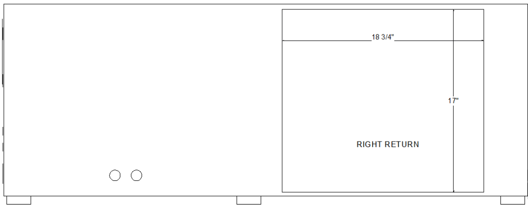
RIGHT VIEW
