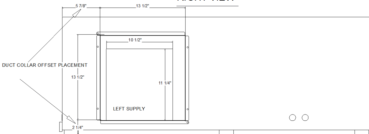
LEFT VIEW
