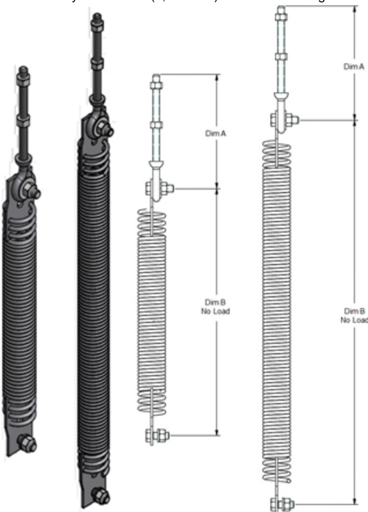
Horizontal Vertical Spring Specifications
