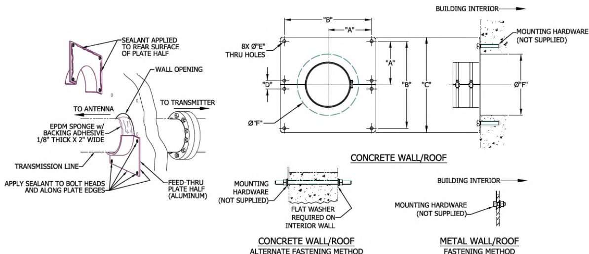
Wall/Roof Feed Thru Plate Specifications
