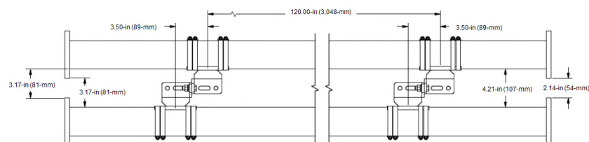
3-1/8-inch Rigid Line
