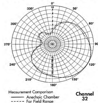
UHF TV Slot Array Azimuth Pattern
