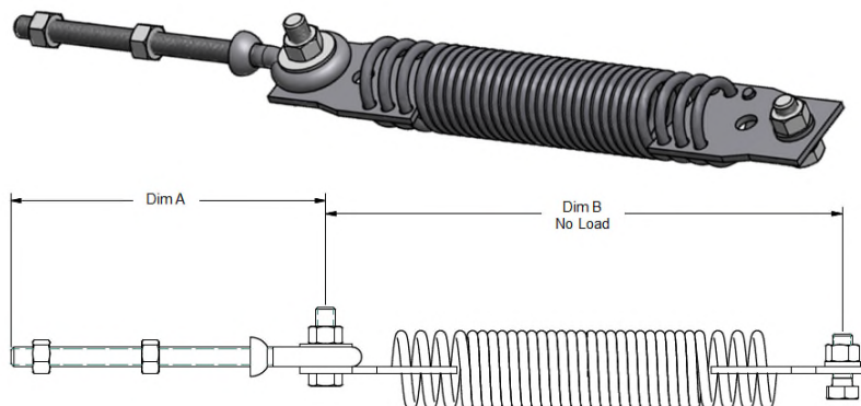
Horizontal Side Spring Specifications
