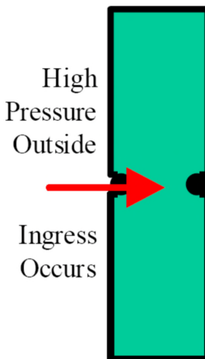
High Pressure System Moves In
