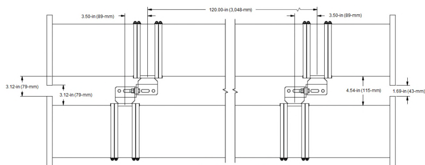
8-3/16-inch Rigid Line
