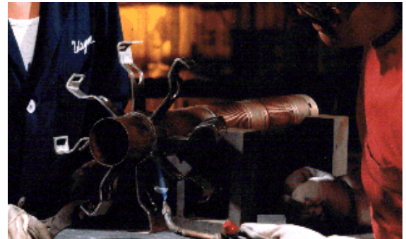
ERI TRASAR Differential Expansion Compensation Assembly
