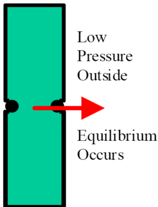
Pressure Equilibrium in Low-Pressure Storm
