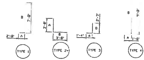
TO BE PLACED IN ALL CORNERS. BENT REBAR DETAIL
