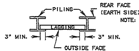
DETAIL 'A-A'
