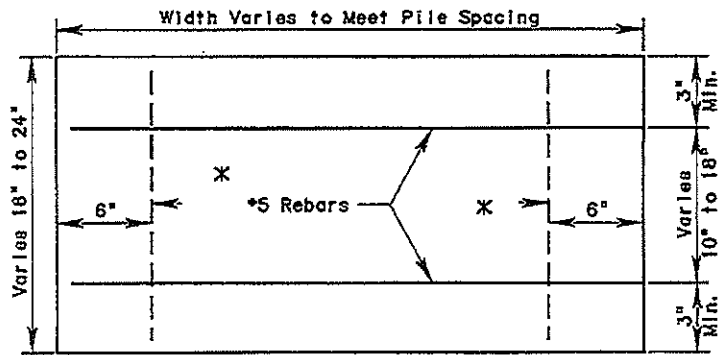
ELEVATION VIEW
