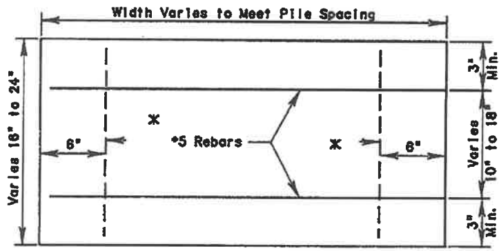
ELEVATION VIEW
