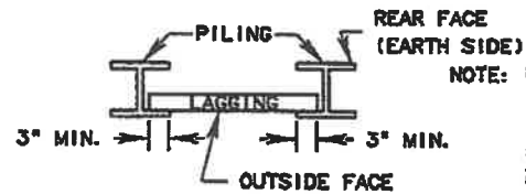
DETAIL 'A-A'
