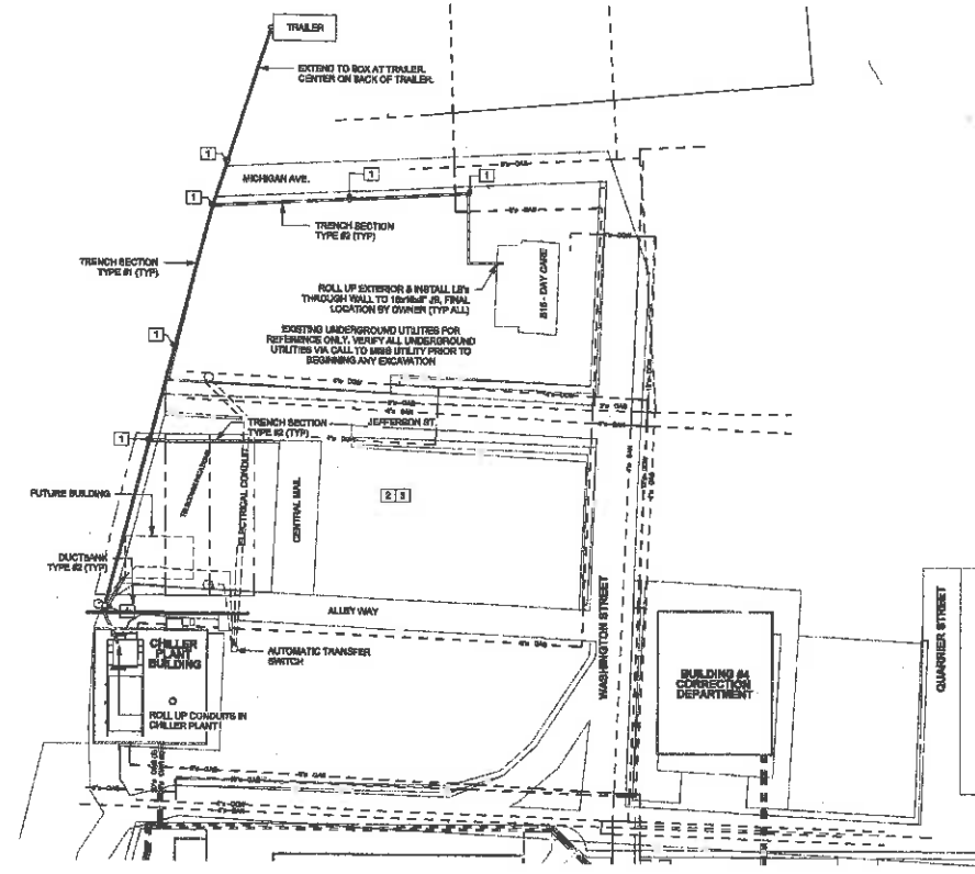
1 EAST CAPITOL COMPLEX TELECOMMUNICATIONS SITE PLAN
