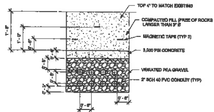
2 TELE/DATA TRENCH SECTION #1
