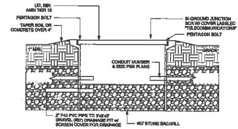
3 IN-GROUND BOX DETAIL
