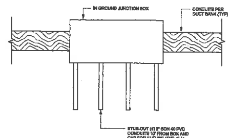
6 IN-GROUND BOX ENLARGED DETAIL (PLAN)
