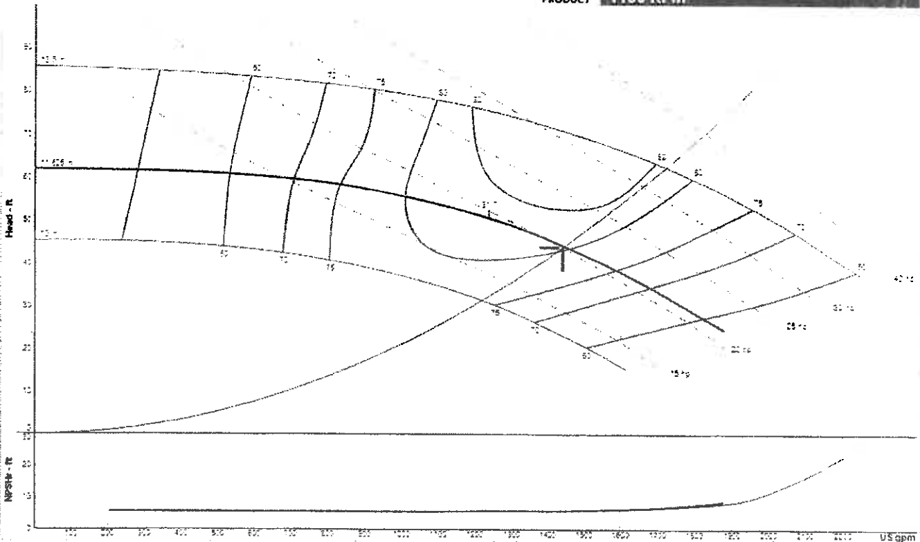
Performance curve meets 14.6 / ISO 9906 acceptance criteria
