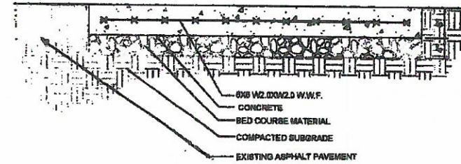
CONCRETE PAVEMENT DETAIL - TYPICAL
