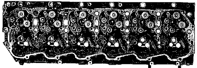
These pictures are from a Cummins ISX engine with 460,913 miles running Shell ROTELLA® T5 Ultra 10W-30. The valve deck received a rating of 9.72 and the Rocker Cover a rating of 9.74 with 10 being clean.
