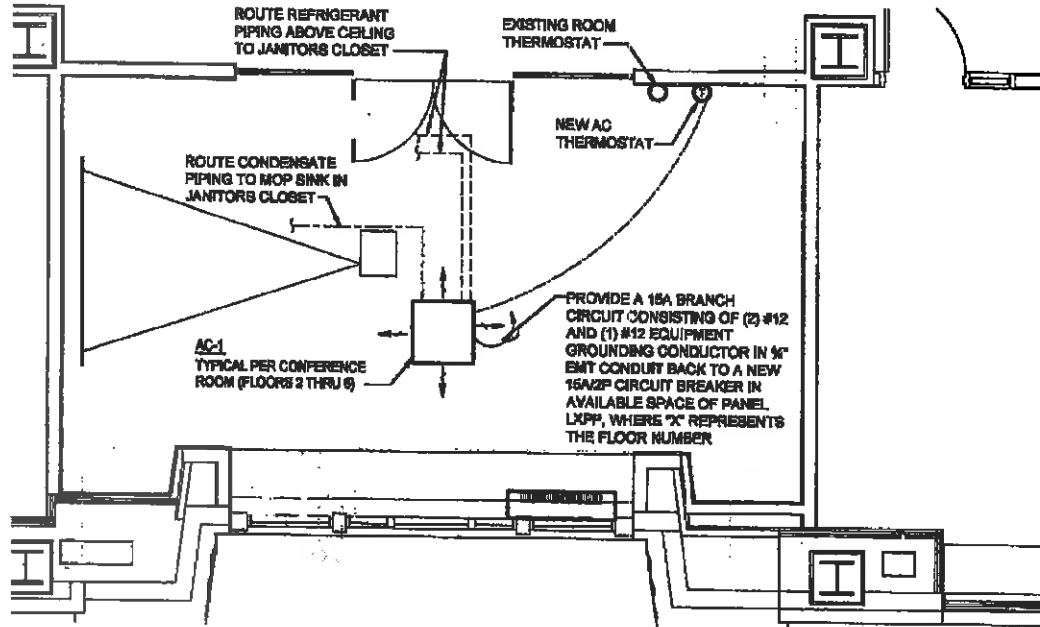
1 TYPICAL CONFERENCE ROOM FLOOR PLAN SK-1 1/4" = 1'-0"
