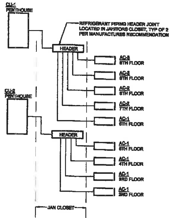
2 UNIT CONFIGURATION SK-3 NTS
