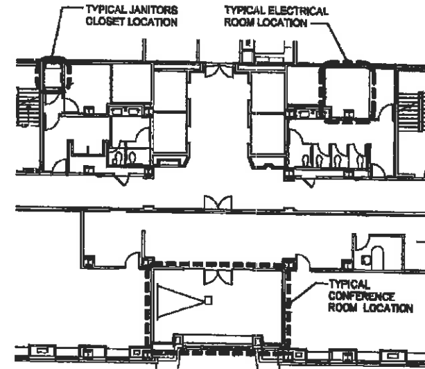
2 TYPICAL FLOOR PLAN SK-1 1/16" = 1'-0"
