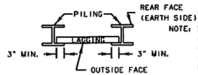
DETAIL 'A-A'
