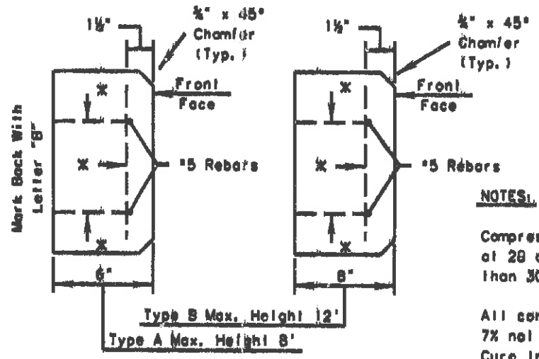
END VIEW
