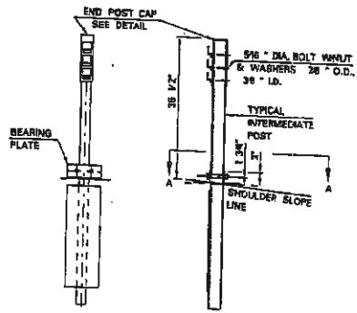
END POST DOUBLE FACE
