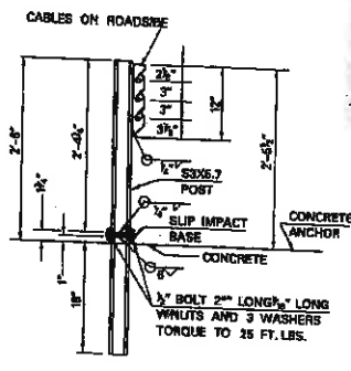
ANCHOR POST DETAIL
