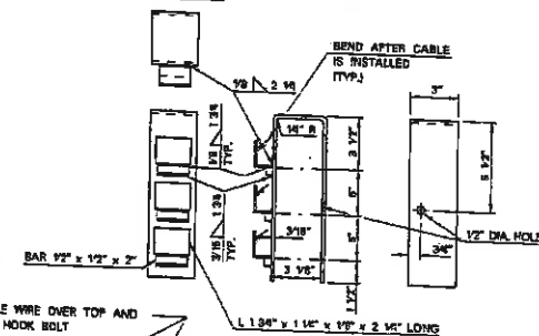
END POST CAP ELEVATION VIEW
