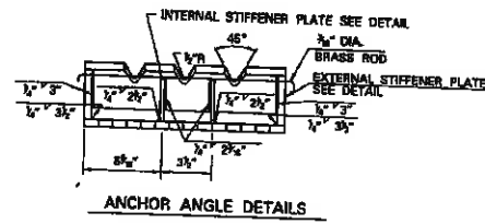
BREAKAWAY ANCHOR ANGLE
