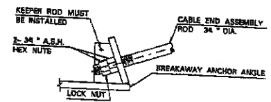
CABLE END ASSEMBLY ROD CABLE TO ANCHOR
