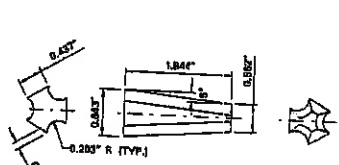
CABLE WEDGE TYPICAL WEDGE FOR ALL SPLICES AND CABLE FITTINGS
