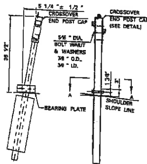
CROSSOVER END POST DOUBLE FACE
