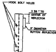
REFLECTOR MOUNT DETAIL ELEVATION VIEW
