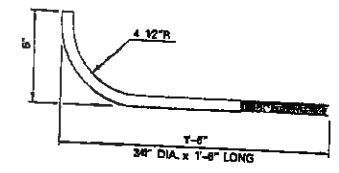
GALVANIZED ANCHOR STUD OPTION
