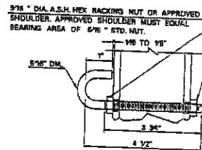
REFLECTOR MOUNT DETAIL PLAN VIEW
