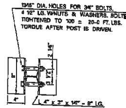
SECTION A-A BEARING PLATE
