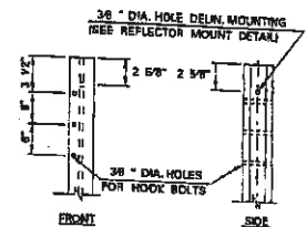
DOUBLE FACE CABLE GUARDRAIL POST HOLE PLACEMENT DETAIL INTERMEDIATE POST
