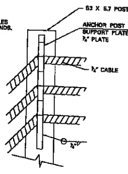
FRONT VIEW OF POST TOP (ROAD SIDE)
