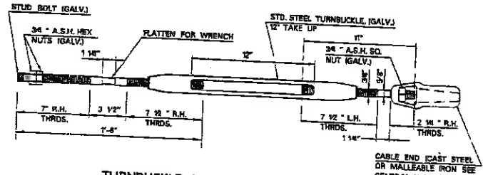
TURNBUCKLE CABLE END ASSEMBLY
