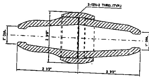
CABLE SPLICE NOTE: USE WITH WEDGE
