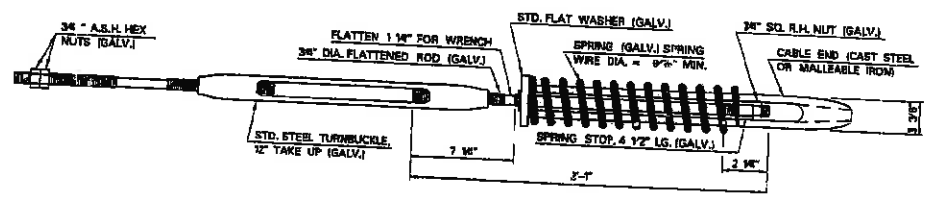
SPRING CABLE END ASSEMBLY COMPENSATING DEVICE
