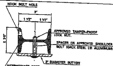
REFLECTOR MOUNT DETAIL PLAN VIEW
