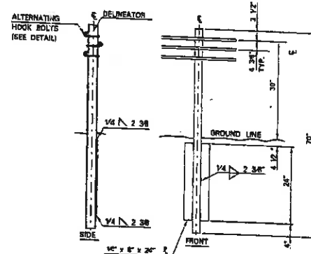
DOUBLE FACE CABLE GUARDRAIL INTERMEDIATE POST
