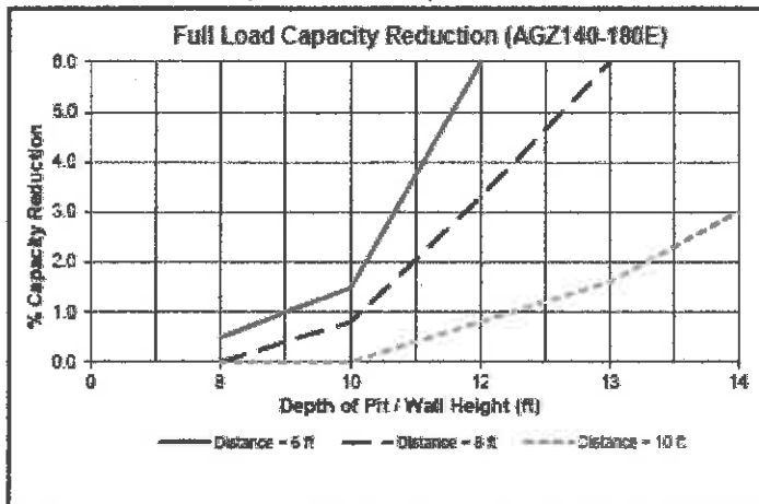
Case 5 - Full Load Capacity Reduction (AGZ140-180E)
