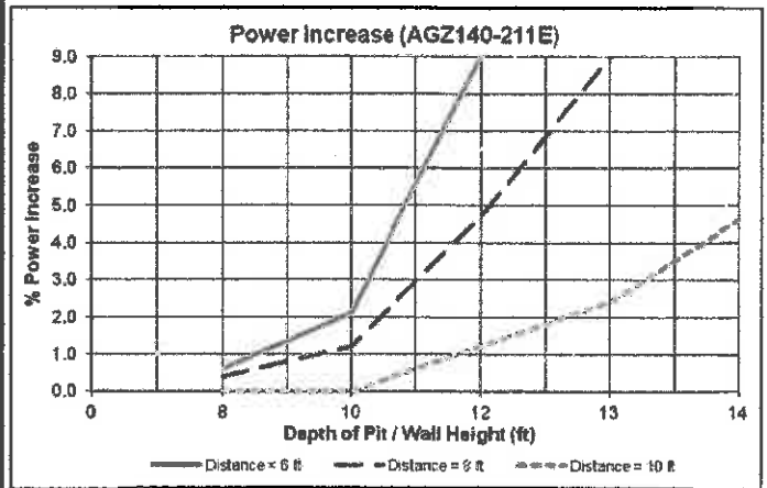
Case 5 - Power Increase (AGZ140-211E)
