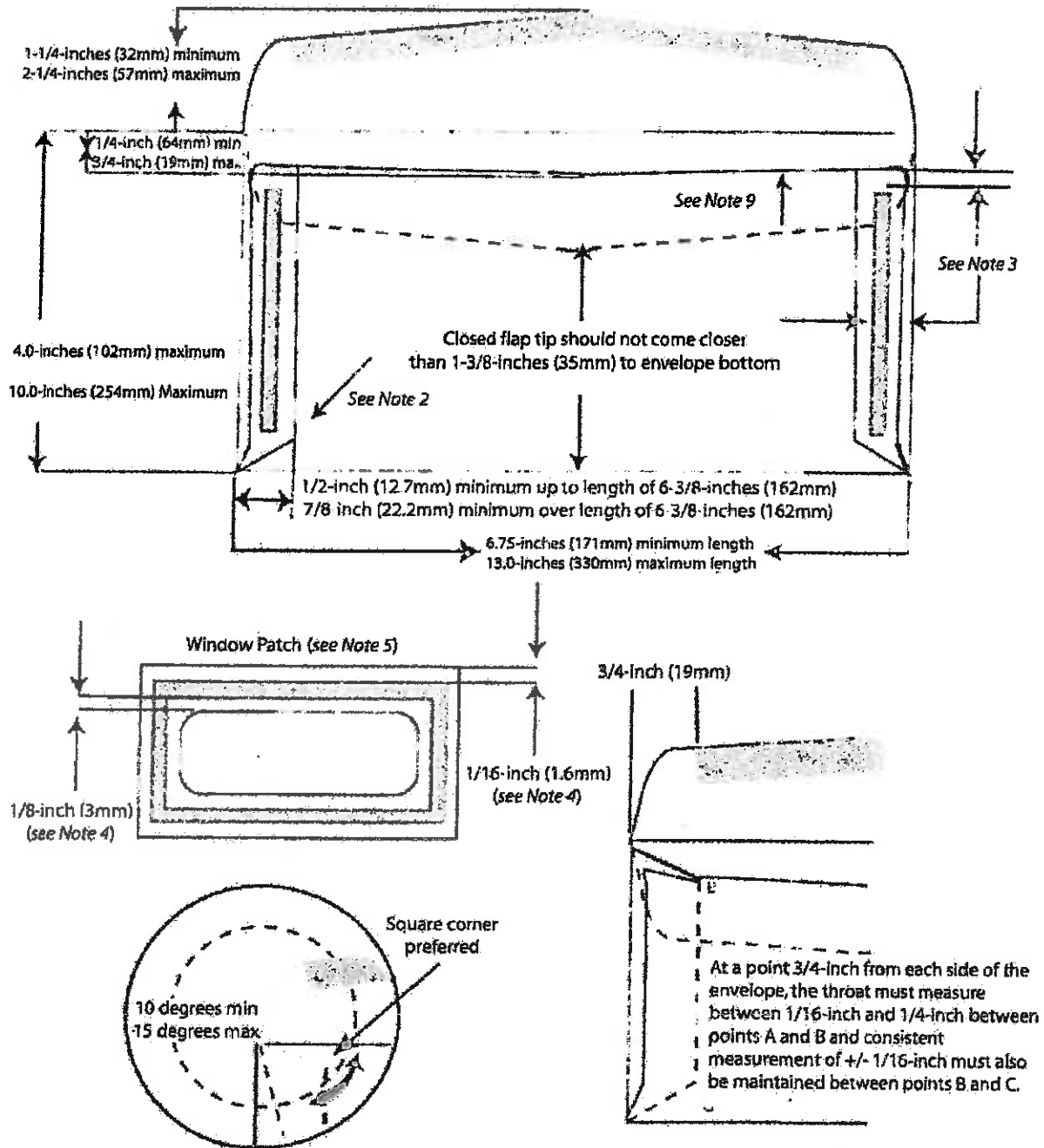
Figure 1-9: Side Seam Envelope Diagram
