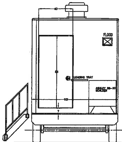
REAR INTERIOR ELEVATION
