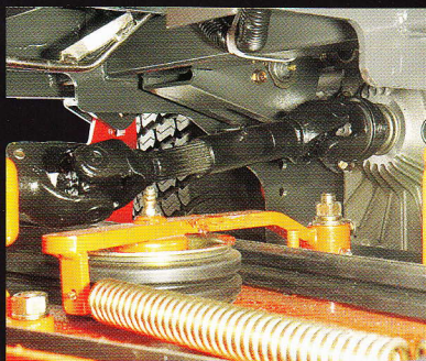
Shaft Drive
