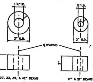
BLOCKOUT DETAILS
