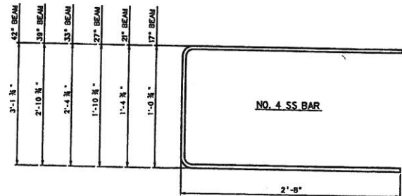
END BEARING DETAIL WITHOUT BACKWALL
