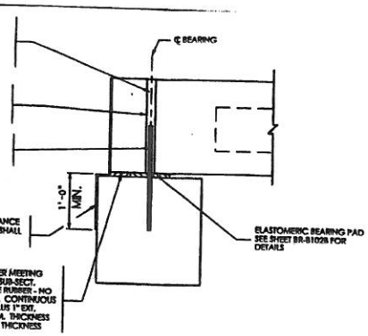
END BEARING DETAIL WITHOUT BACKWALL
