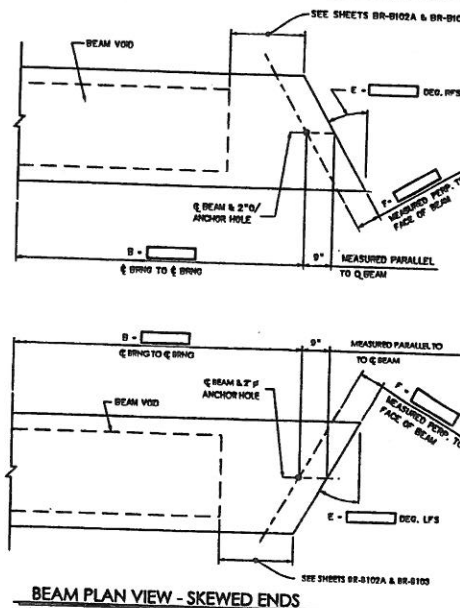
BEAM PLAN VIEW - SKEWED ENDS
