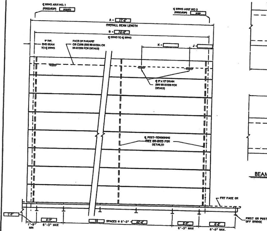
DECK PLAN VIEW
