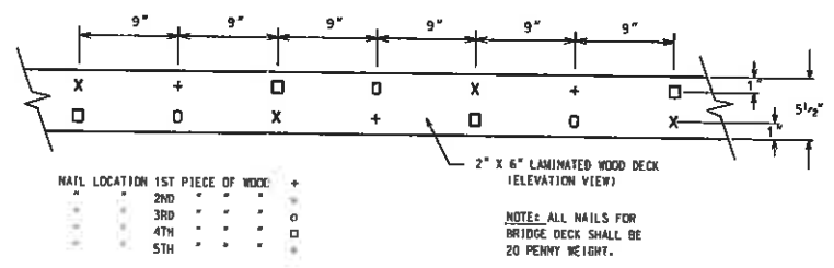
TIMBER DECK NAILING DIAGRAM NO SCALE
