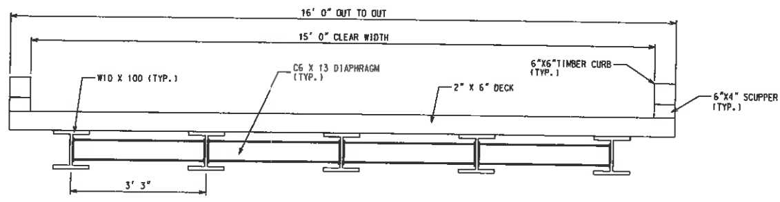
DECK SECTION
