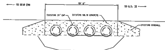
EXISTING ELEVATION VIEW NO SCALE
