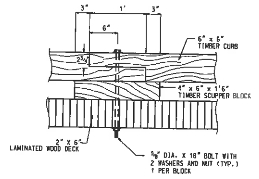
CURB SPLICE DETAIL A
