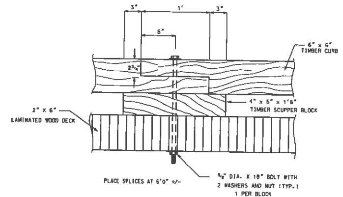
CURB SPLICE DETAIL NO SCALE
