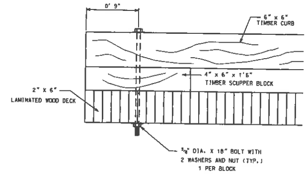
CURB END DETAIL NO SCALE
