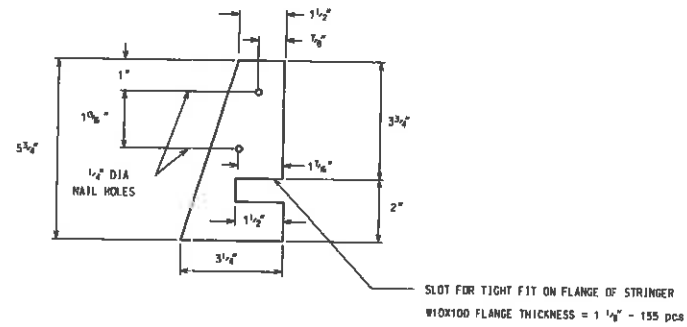
DECK ANCHOR PLATE DETAILS NO SCALE
