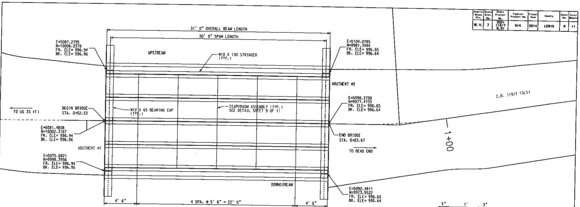
STEEL LAYOUT
