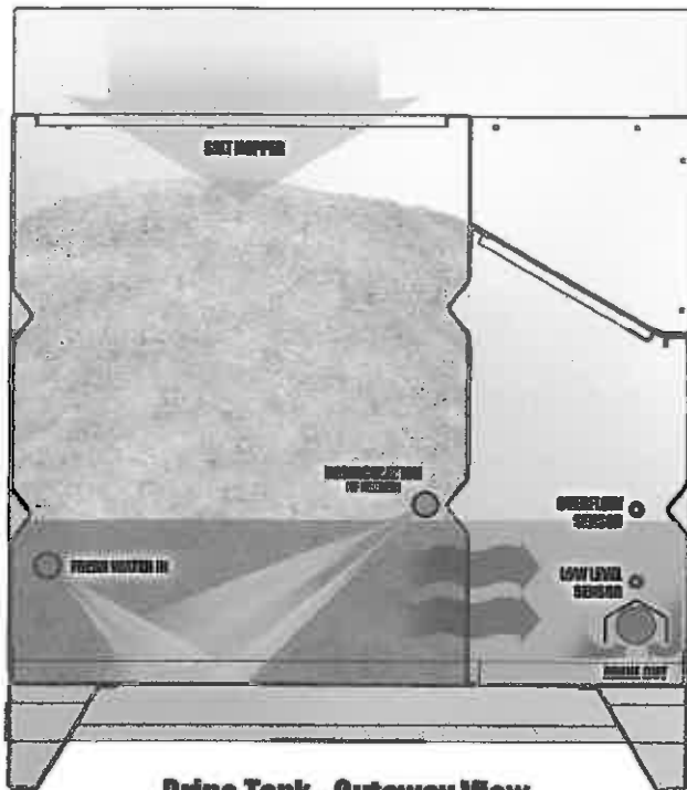
Brine Tank - Cutaway View
