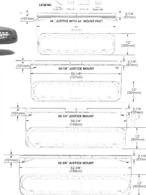
JUSTICE DIMENSIONS & LIGHTHEAD POSITION DIAGRAM
