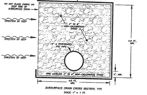
DETAIL 21 SUBSURFACE DRAIN DETAILS SCALE: AS NOTED
