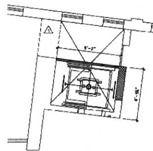
D PLAN ELEVATOR "A" SCALE: 1/4"=1'-0"
