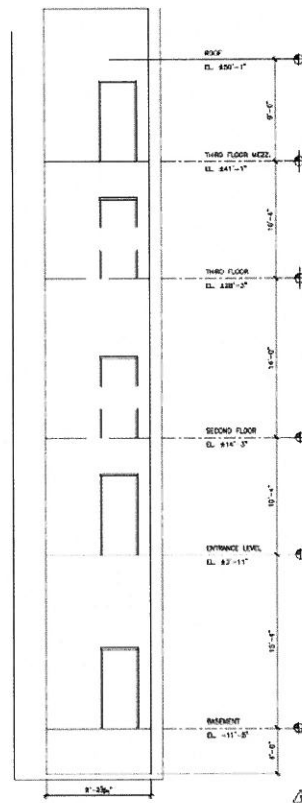
A SECTION THRU ELEVATOR "A" SCALE: 1/4"=1'-0" NOTE: SEE ELEVATOR DATA SHEET FOR #1
