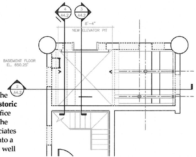
1 BASEMENT ELEVATOR PLAN SCALE: 1/4"=1'-0"
