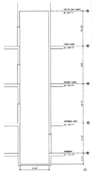
B SECTION THRU ELEVATOR "B" SCALE: 1/4"=1'-0" NOTE: SEE ELEVATOR DATA SHEET FOR #1
