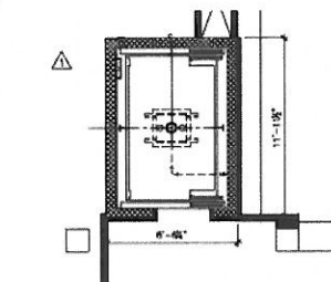
C PLAN ELEVATOR "B" SCALE: 1/4"=1'-0"
