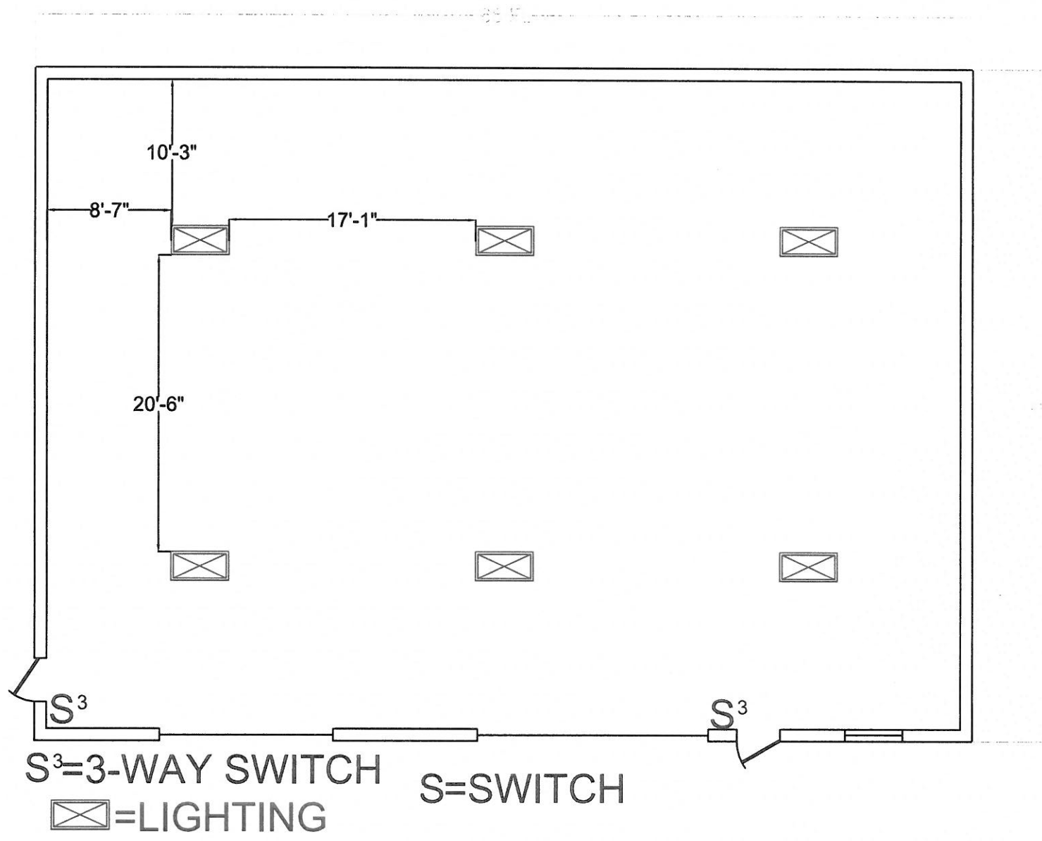
LIGHTING LAYOUT WVDA DRAWINGS No.3
