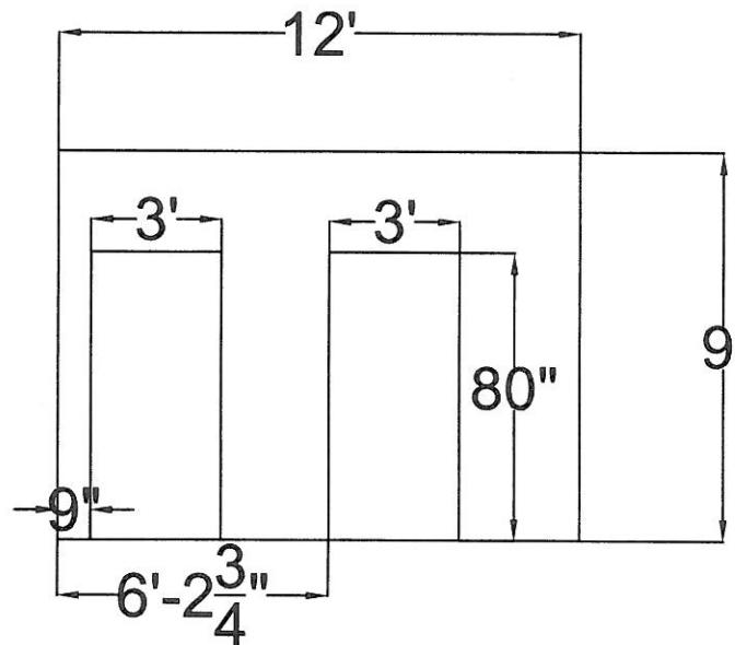
OFFICE WEST WALL ELEVATION WVDA DRAWINGS No.8
