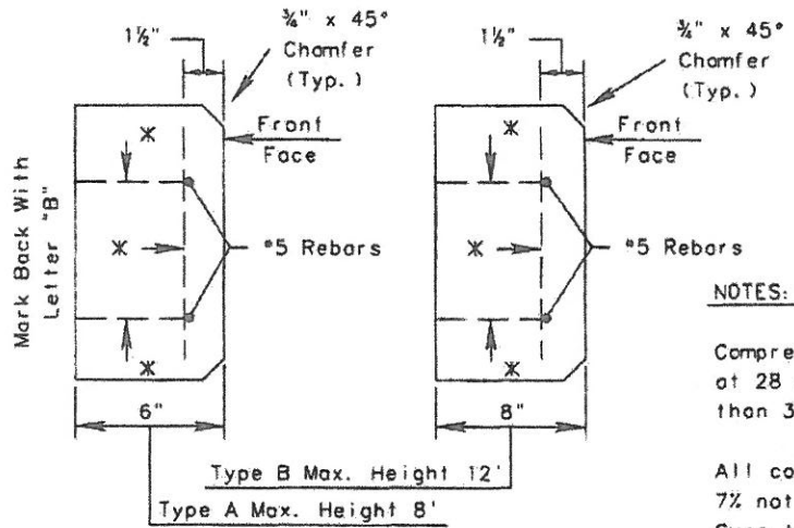
END VIEW
