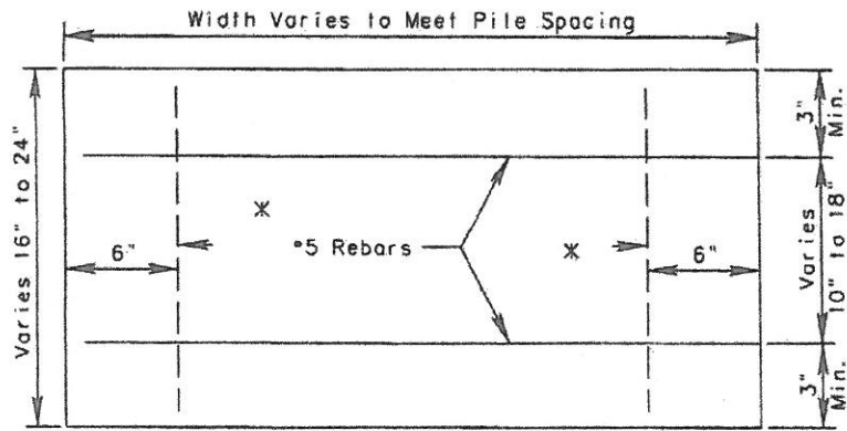
ELEVATION VIEW
