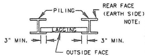
DETAIL 'A-A'
