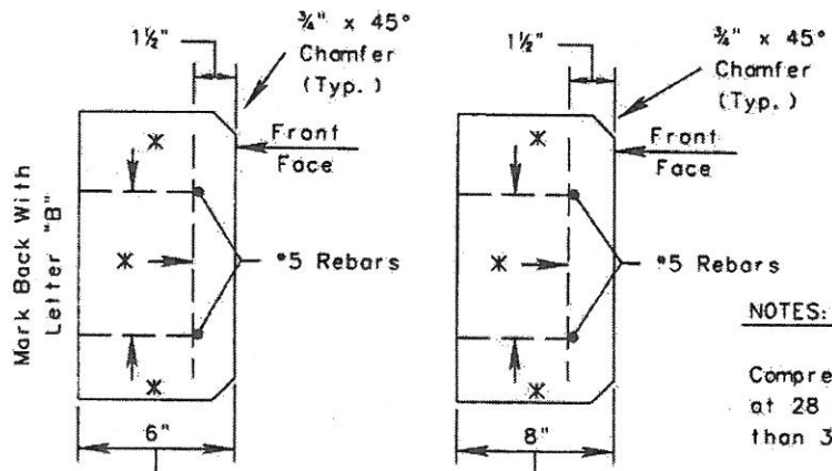
ELEVATION VIEW
