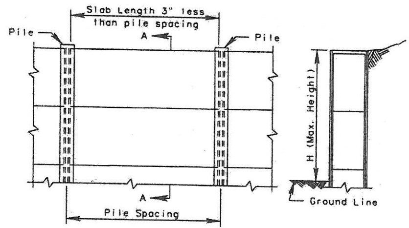
ELEVATION OF WALL
