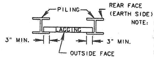
DETAIL 'A-A'
