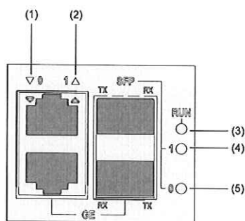
Figure 2 FIP-210 LEDs
