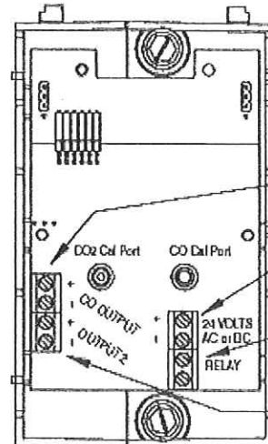
Duct Mount
