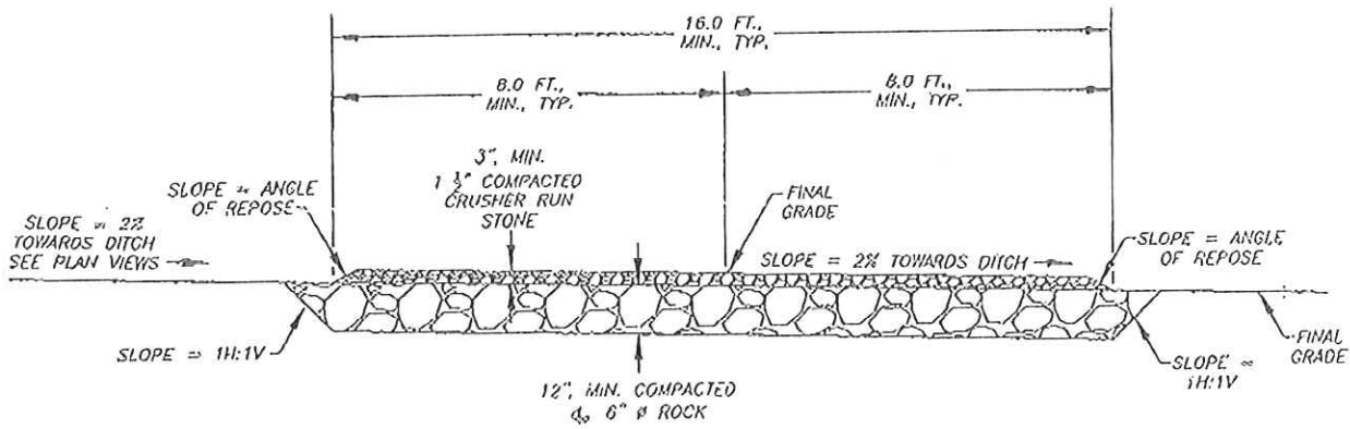
DETAIL 34 CONSTRUCTED ACCESS ROAD, TYP.
