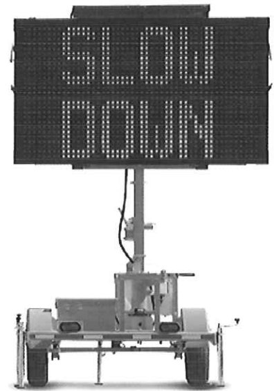
Mini Matrix Sign WVTM(A) Hydraulic lift WVTM(B) Manual winch
