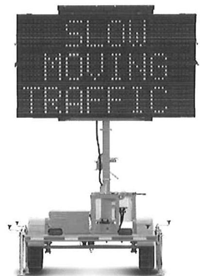
Mini Three-Line Sign WVT3(A) Hydraulic lift WVT3(B) Manual winch
