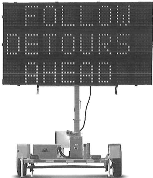
Three-Line Sign WTLMB-(A) Hydraulic lift WTLMB-(B) Manual winch
