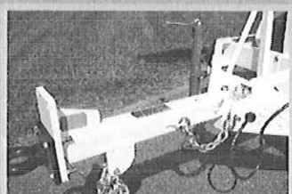
Telescopic tongue with height-adjustable pintle ring
