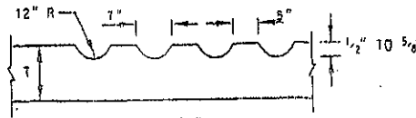
SECTION C-C (MILLED RUMBLE STRIP)
