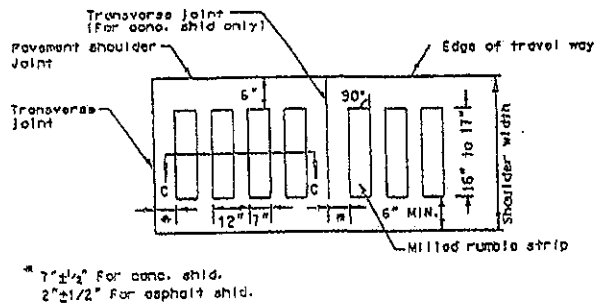
MILLED RUMBLE STRIP FOR PORTLAND CEMENT AND HOT MIX ASPHALT SHOULDERS
