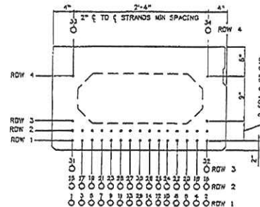
BEAM PRESTRESSING TYPICAL BEAM END & MIDSPAN
