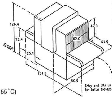
Dimensions are in centimeters Note: Non-marring castors
