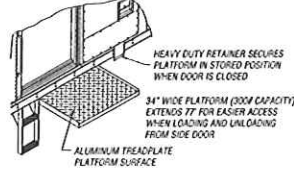
Steel Stirrup Step with Slide-Out Platform
