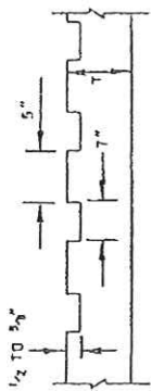
ALTERNATE SECTION 8-B (SAWED RUMBLE STRIP)
