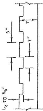
ALTERNATE SECTION B-8 (SAVED RUMBLE STRIP)
