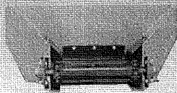
7 Gauge, Replaceable Chain Shields 10 Gauge Hopper
