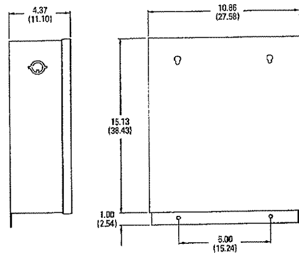
MCS16-10
