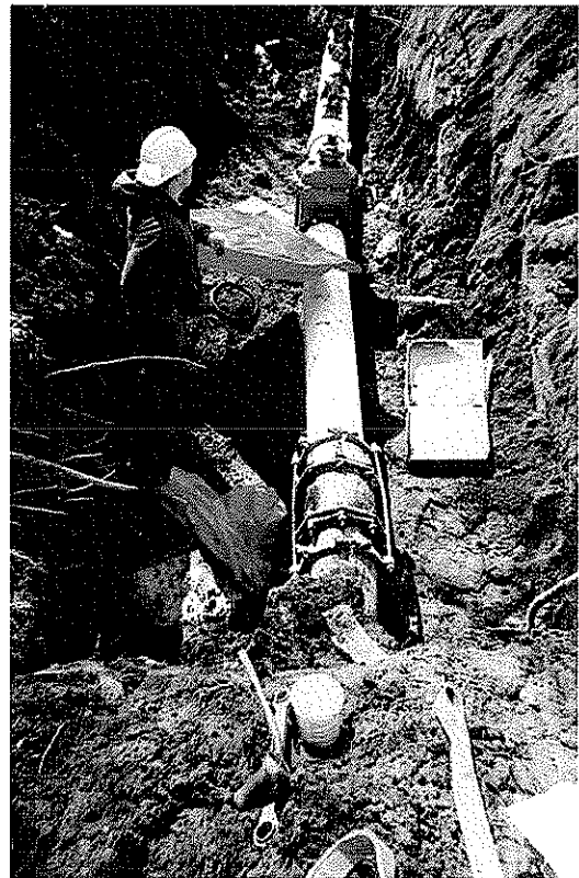
Connection of 10" HDPE River Crossing Pipe (Directionally Drilled) to 10" C-900 Pipe at Tygart Valley River
