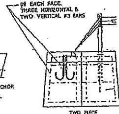
ANCHOR UNIT & RE-BAR INSTALLATION DETAIL
