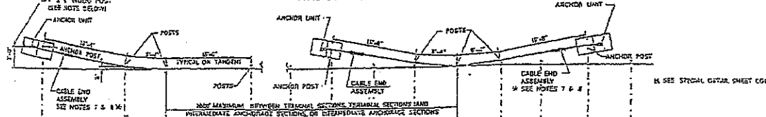
PLAN TYPICAL APPROACH & TERMINAL SECTIONS
