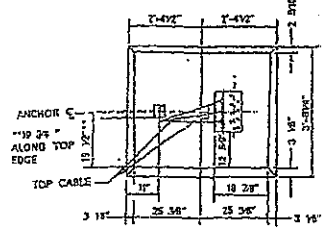
ANCHOR UNIT DETAIL TOP VIEW RIGHT HAND (REINFORCEMENT NOT SHOWN)
