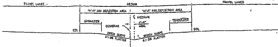
TYPICAL SECTION (DEFLECTION AREA ON MEDIAN SLOPES) DOUBLE FACE GUIDERAIL APPLICATION
