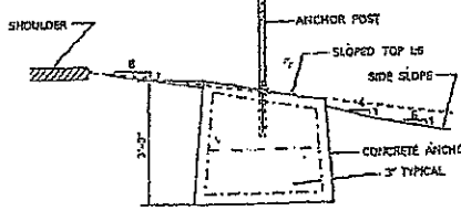
ANCHOR UNIT & RE-BAR INSTALLATION DETAIL
