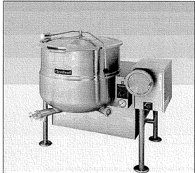
Shown with optional Spring Assisted Cover and 2" Tangent Draw-Off Valve
