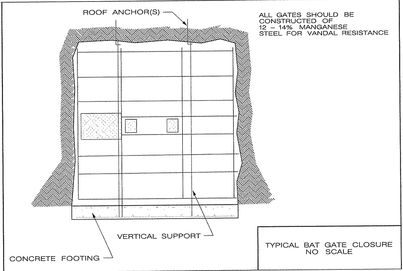
Figure 7—Typical Bat Gate Closure for Unstable Mine Highwall
