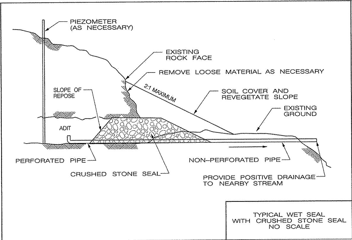
Figure 6—Typical Wet Seal Portal Closure
