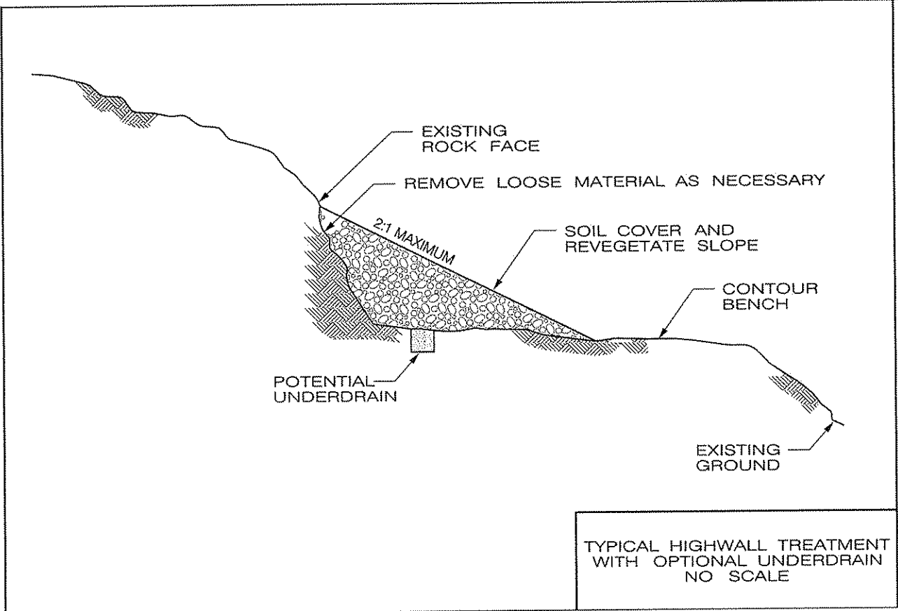
Figure 8—Typical Mine Highwall Stabilization
