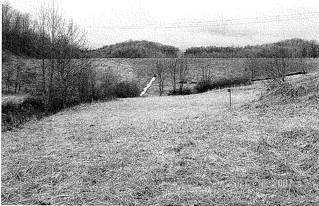
LEMLEY DAM MODIFICATION, MONONGALIA CO., WV
