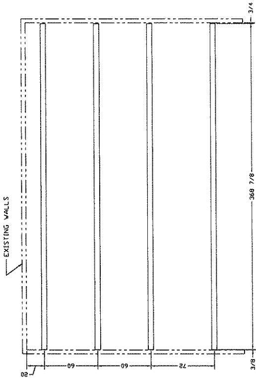
RAIL "MODULAR DECK" ARRANGEMENT
