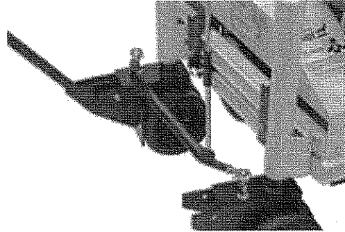
Steering handle, brake, tie rod and pointer arm
