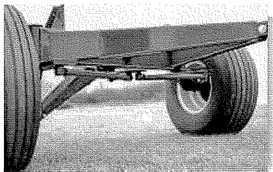
Tapered Ball Joint Automotive Type Steering and replaceable bronze bushings at all pivot areas have grease fittings at all pivot points. Tapered heat treated sleeves welded to the steering arms minimize loosening wear.
