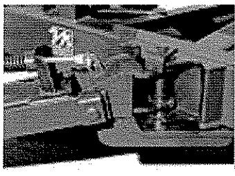
Machined pivot pins versus bolts insure continued close tolerances. All pivot pins are set in replaceable bronze bushings with grease fittings for longer life.
