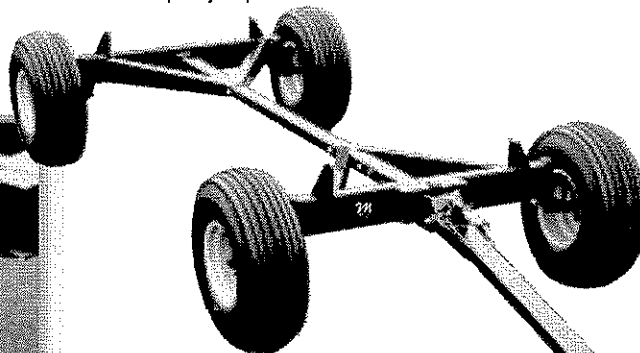
Single rear axle models 12T-8, 15T-8 and 17T-8 are rugged, yet economical.
