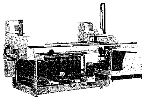
JANUS 2-arm Automated Workstation with Integrator deck, 8-tip dispense arm and labware movement tool shown interfaced to a Victor™ plate reader.
