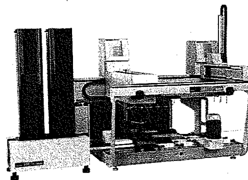
Enhanced capacity is achieved by integrated up to four PlateStak Microplate Storage Devices providing up to 200 additional microplates or over 50-tip box capacity.
