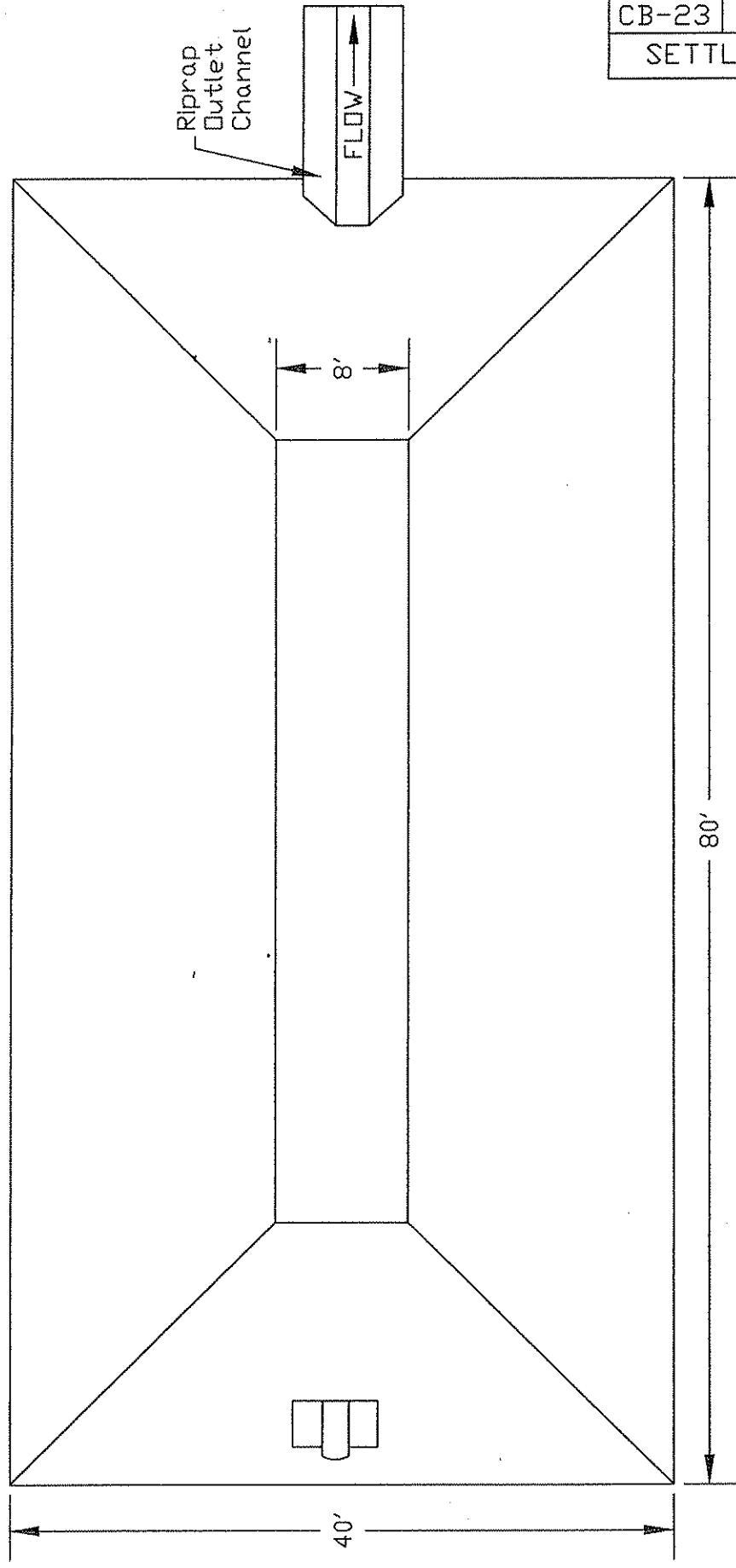
PLAN VIEW
